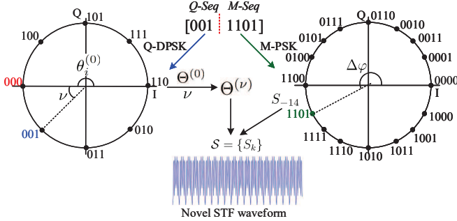
Fig. 3. Preamble modulation.
