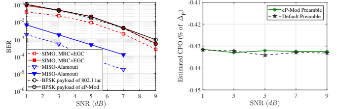
Fig. 9. BER and CFO in USRP experiments, eP\text{-Mod}(Q = 64, M = 16) . (a) BER of eP\text{-Mod} vs BPSK payload. (b) Average of estimated CFO.
