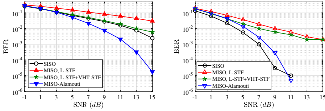
Fig. 6. BER of eP\text{-Mod} for MISO vs. SISO, Rayleigh channel (simulations). (a) eP\text{-Mod}(Q = M = 32) . (b) eP\text{-Mod}(Q^*, Q = 32) .
