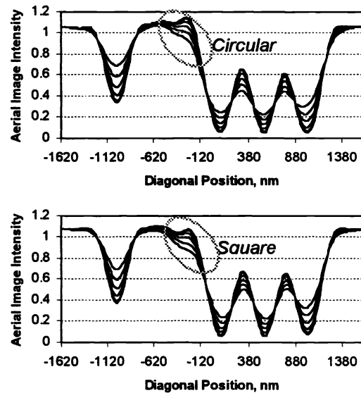
Figure 7. 2D image comparisons for a diagonal cut-line through elbow pattern for circular and square source shapes.
