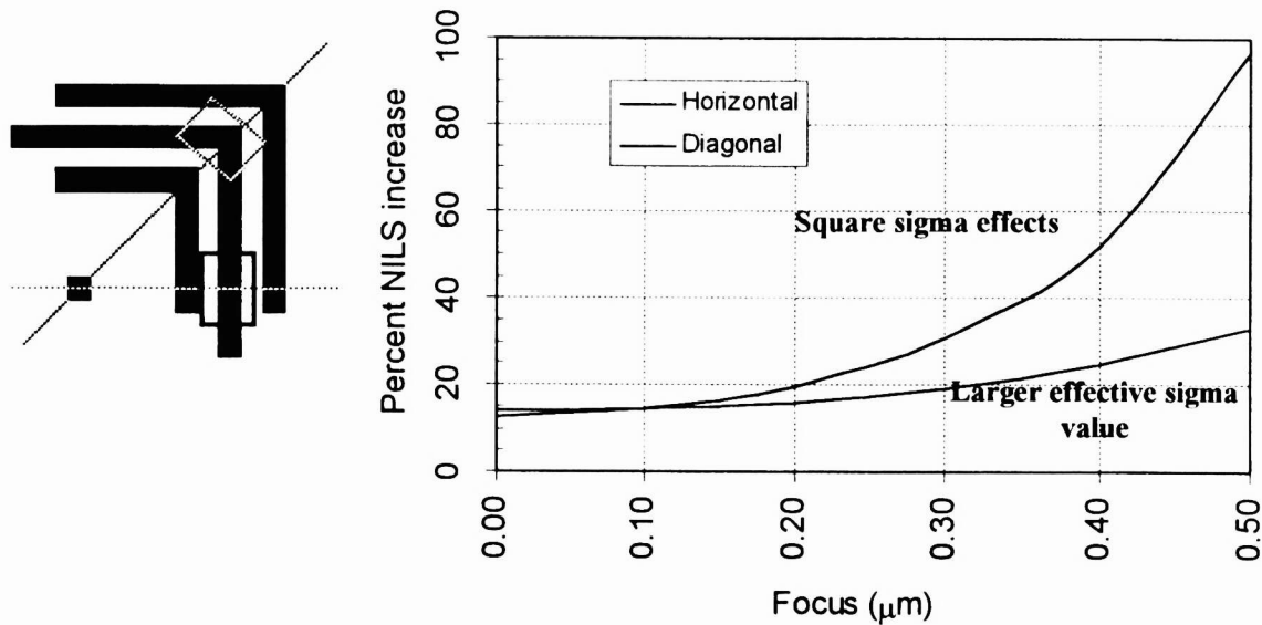
Figure 8. The improvement with square shape over circular, measured in terms of NIS increase, for horizontal and diagonal orientations.
