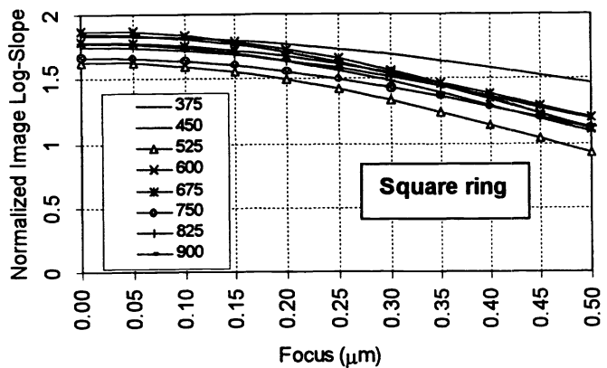
Figure 14 Annular vs. square ring performance measured as NILS through focus and pitch. Wavelength is 248 nm with a 0.63 NA for 150 nm features with duty ratios from 1:1.5 to isolated.
