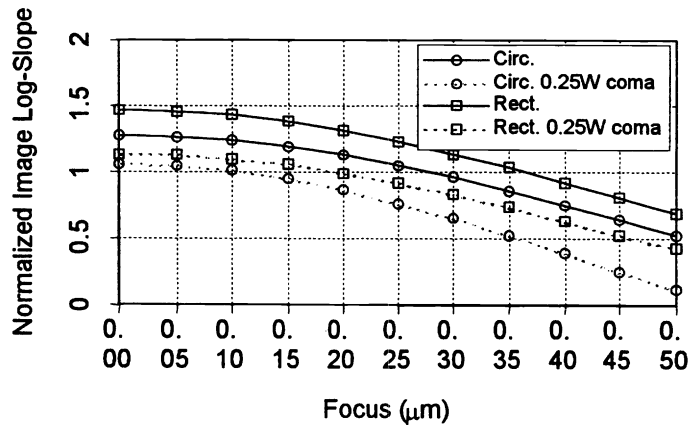
Figure 11. Effects of coma on NILS for circular and square (rectangular) source shapes.
