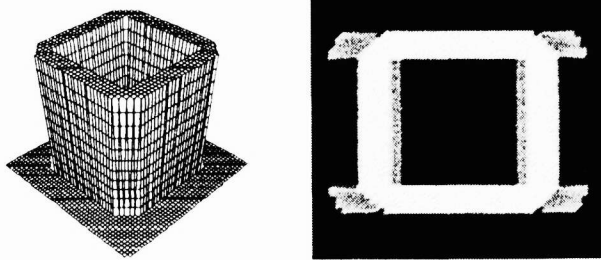
Figure 13. A square-ring annulus shape for off-axis illumination. This source is optimized for k_1 near 0.40. Maximum overlap of diffraction orders is achieved, which is superior to circular-ring annular illumination.
