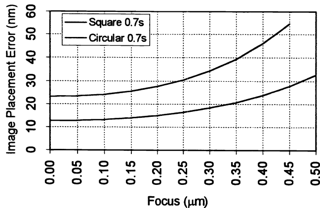
Figure 12. Effects of coma on IPE for circular and square source shapes (0.25 waves of primary coma).
