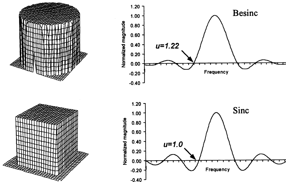
Figure 1 Circular and square shaped pupils and their corresponding transforms.
