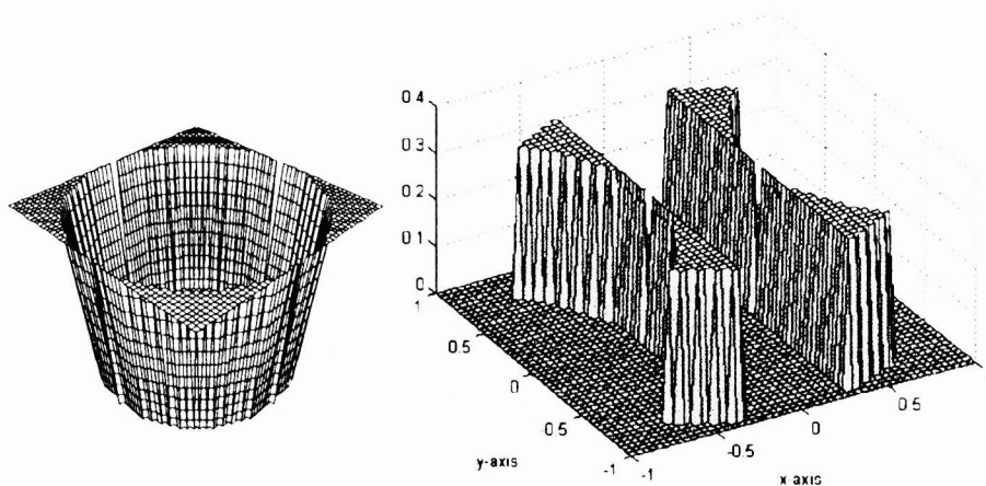
Figure 4. The effects of overfilling the objective lens with a “difference” pupil and \sigma > 1.0
