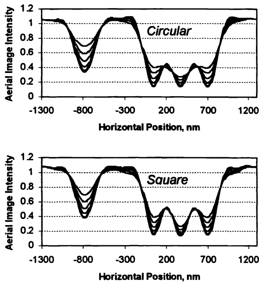
Figure 6. 2D image comparisons for a horizontal cut-line through elbow pattern for circular and square source shapes.
