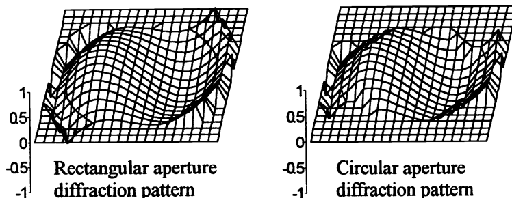
Figure 10 Impact of illumination on coma aberration effects. The diffraction field is plotted for k_1=0.38 with \sigma = 0.7 and 0.25 waves of primary coma.
