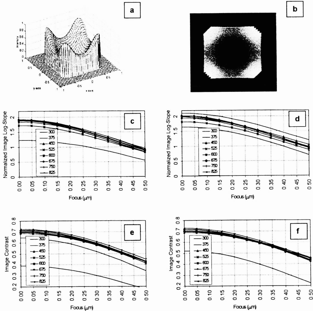
Figure 15. Image performance of a 248 nm, 0.60 NA system for 150 nm lines evaluated using NILS and image contrast. The layout of the source distribution is shown in a and b. Performance of a more conventional Gaussian weak quadrupole source is shown in c and e. Performance of the square-character weak off-axis source is shown in d and f.
