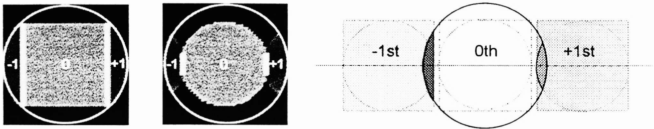
Figure 3 Frequency distribution of diffraction orders in the objective lens pupil for square and circular shaped illumination. Collection of first order is increased for square illumination.
