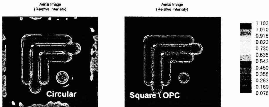
Figure 9. Comparison of 2D aerial images for circular pupil illumination and square pupil illumination with 50 nm serif OPC. Partial coherence for each case is 0.70. Improvements over circular illumination are present in X/Y and diagonal orientations as well as at corners.
