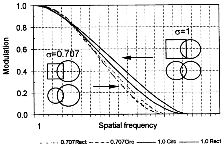
Figure 2. OTF for square and circular pupils illuminating a circular objective lens pupil. Geometry is oriented along X/Y directions and \sigma=1 corresponds to equivalent size condenser and objective lens NA values.
