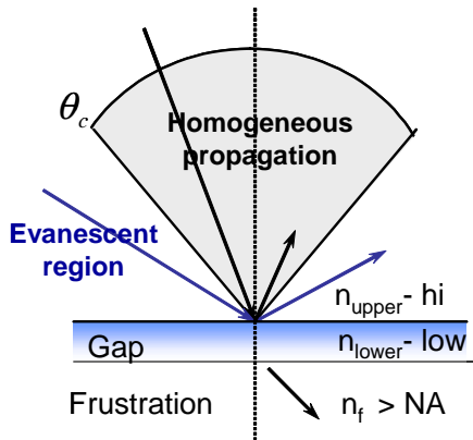
Figure 2. Frustrated total internal reflection (FTIR) of an evanescent field into a media with refractive index larger than the numerical aperture of the propagating wavefront.
