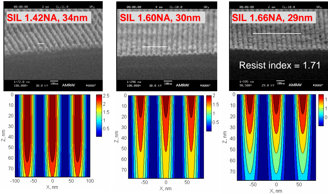
Figure 6. Solid immersion lithography results using the sapphire imaging system (left) 1.42NA for 34nm half-pitch imaging; (middle) 1.60NA for 30nm half-pitch imaging; and (right) 1.66NA for 29nm half-pitch imaging in 78nm photoresist along with ILSim simulations.
